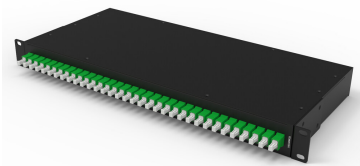
1RU panel, 1X32 split ratio, 1 splitter, LC/APC connectors
