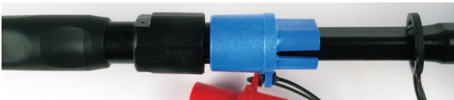
Cleaning Tool Pushed into HMFOC Non-Pinned Connector
