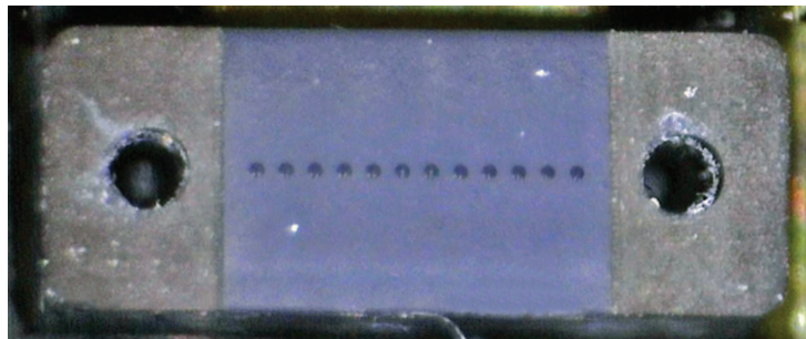
Example of HMFOC Endface with Dirty Pinholes
